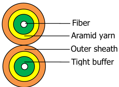
Structural Diagram
